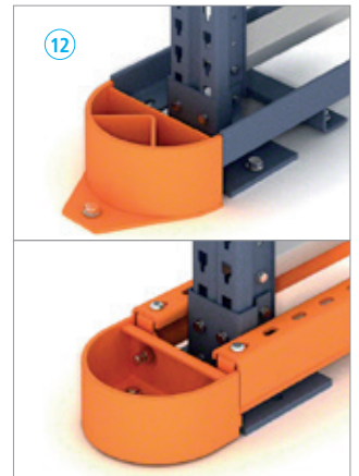
Guide rail and protector
